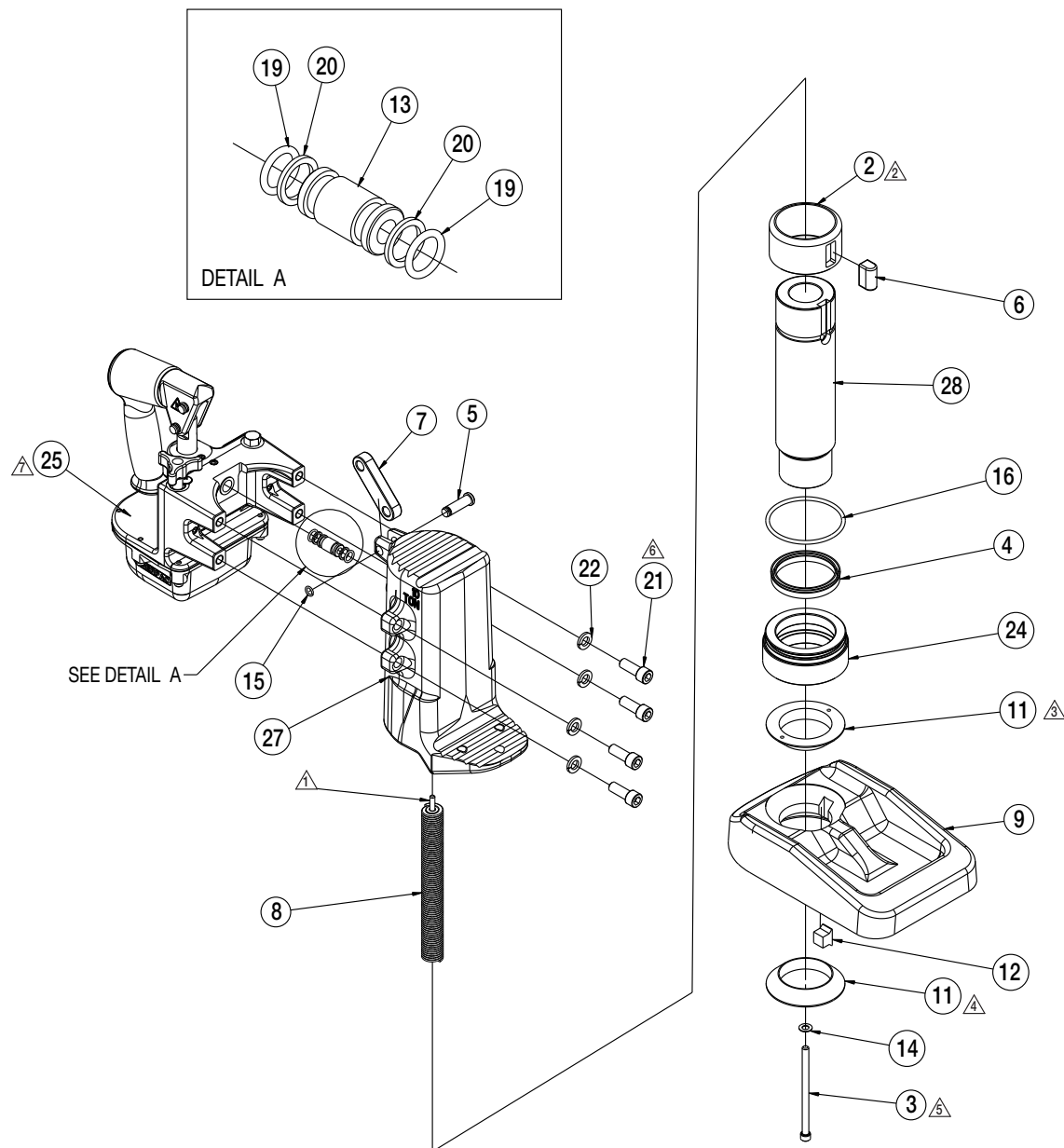
Figure 2 - Main Assembly (View 2 of 2)
