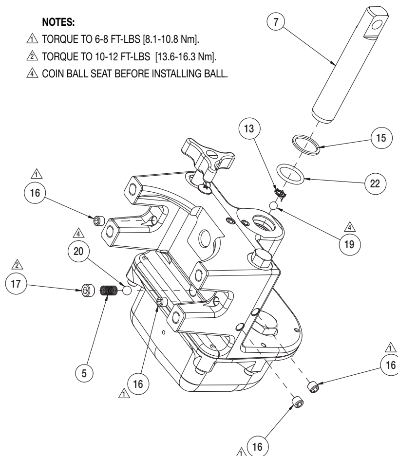
Figure 4 - Pump Assembly (View 2 of 2)
