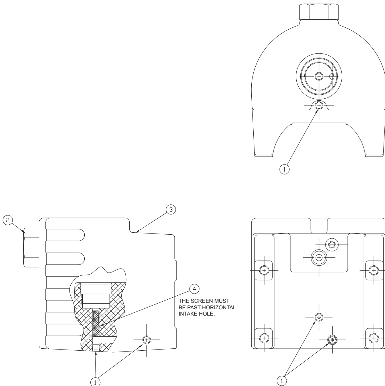
Figure 2 - 40409SR Pump Body Assembly
