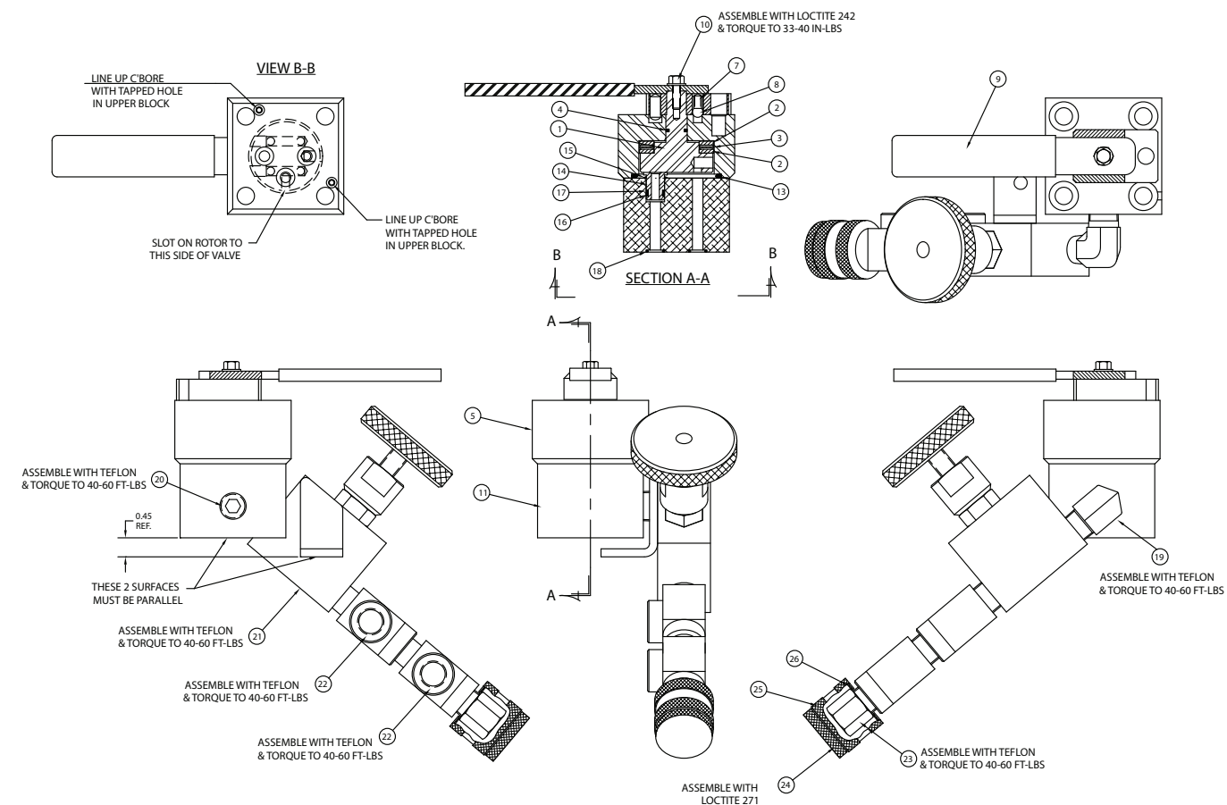
Figure 5 - 46066SR Control Valve Subassembly
