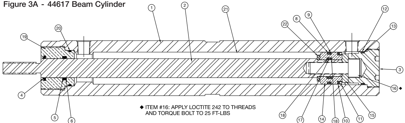
Figure 3A - 44617 Beam Cylinder
